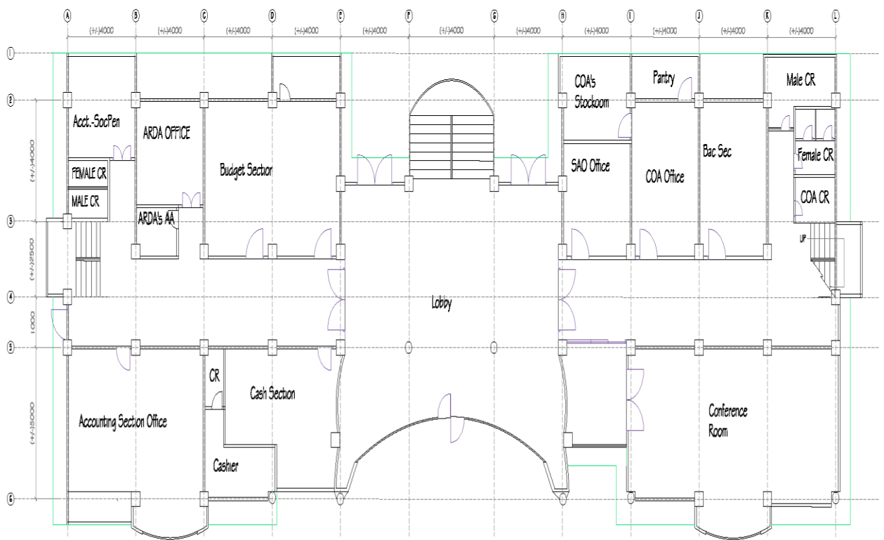
MAIN BUILDING FIRST FLOOR PLAN
