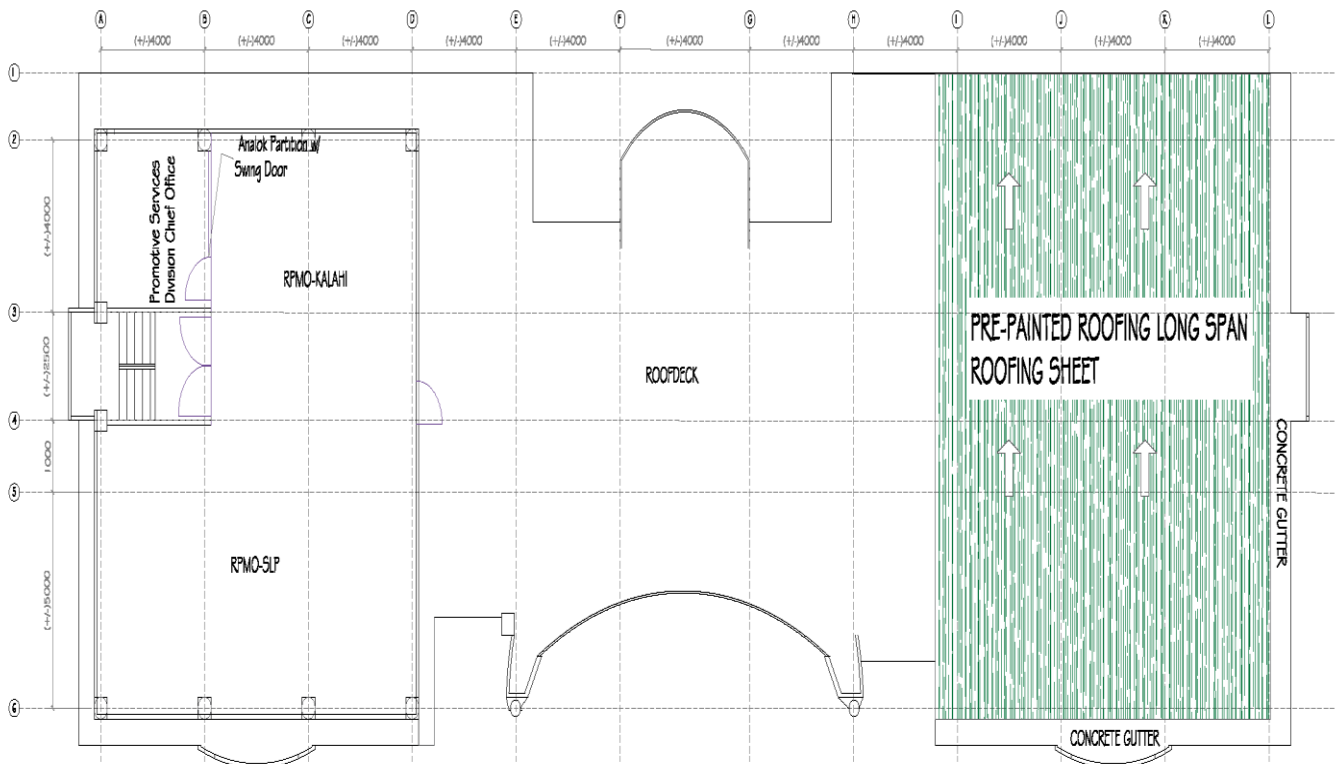
MAIN BUILDING THIRD FLOOR PLAN
